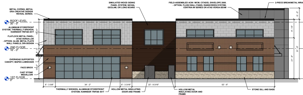
2 SOUTH ELEVATION 1/8" = 1'-0"
